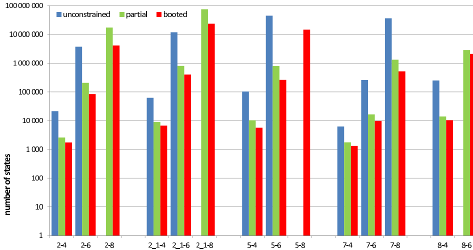
Figure 6: Number of states for some selected scenarios; the x-axis is labeled with a subset of the scenarios of Table 1, where “ s-N ” stands for scenario s for N processors and “ s_{\mathcal{I}}-N ” stands for scenario for s_{\mathcal{I}} for N processors; the repartition between processors with bitstream and vector extension is as indicated in Table 1, i.e., for N = 4 we have N_b = 1 and N_v = 3 , for N = 6 we have N_b = 2 and N_v = 4 , and for N = 8 we have N_b = 2 and N_v = 6
