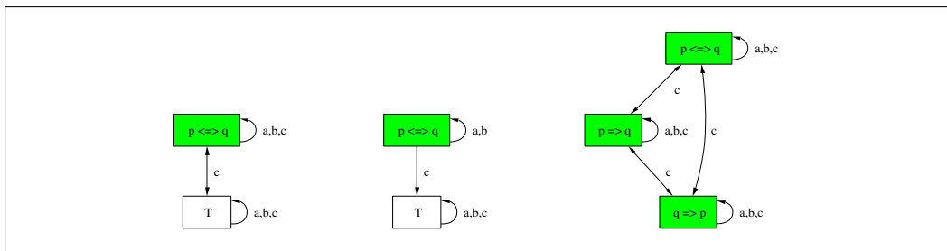
Figure 2. The three action primitives, randomly instantiated. A group announcement to a, b that p \Leftrightarrow q holds, a secret announcement to a, b that p \Leftrightarrow q holds and a group announcement to a, b that one of the choices expressed by the formulas p \Rightarrow q, p \Leftarrow q, p \Leftrightarrow q has been taken. These primitives can be instantiated by using the LYS command amnew (generate a new action model) with the flags -group , -secret and -choice , respectively.
