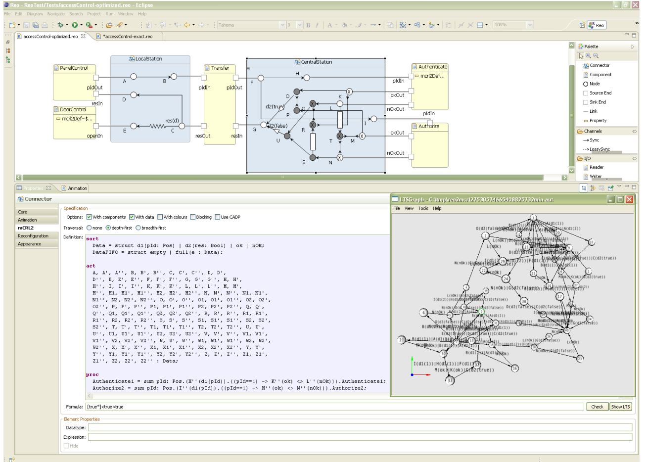
Fig. 15. Extensible Coordination Tools: Reo to mCRL2 plug-in
