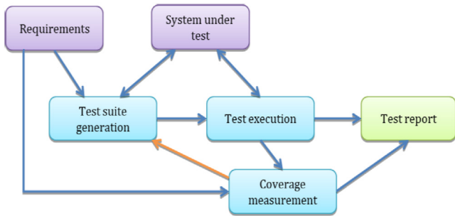
Fig. 10. Requirements-based testing.
