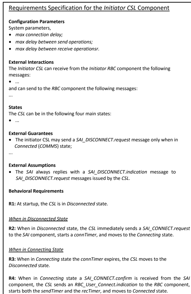
Fig. 9. Natural Language requirements for ICSL
