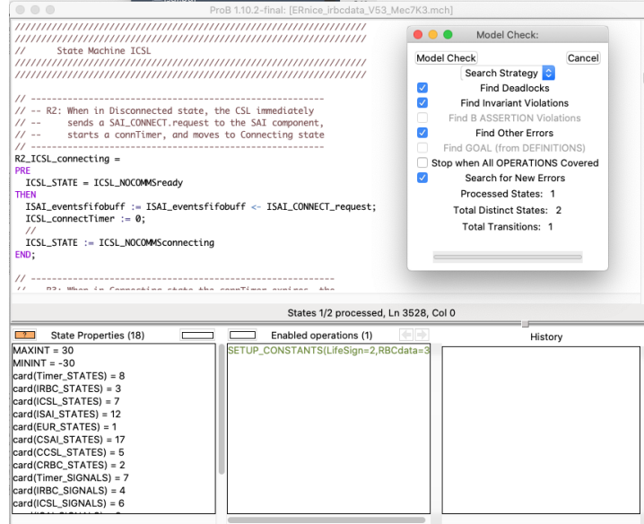
Fig. 8. Model Check GUI of ProB
