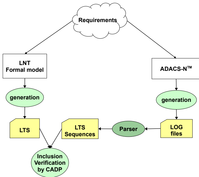
Figure 10: The approach applied to ADACS-N TM validation
