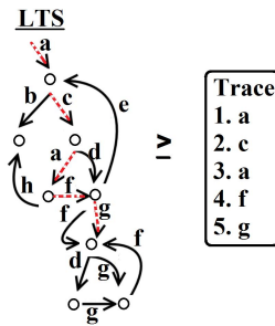
Figure 4: Example of trace inclusion checking
